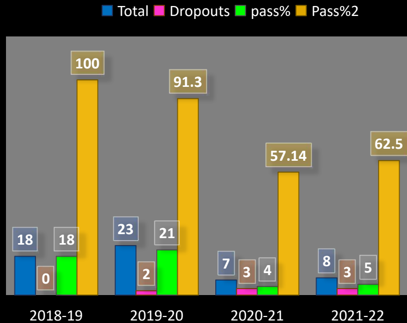
ACADEMIC RESULT OF PG FROM SESSION 2018-19 TO 2021-22
