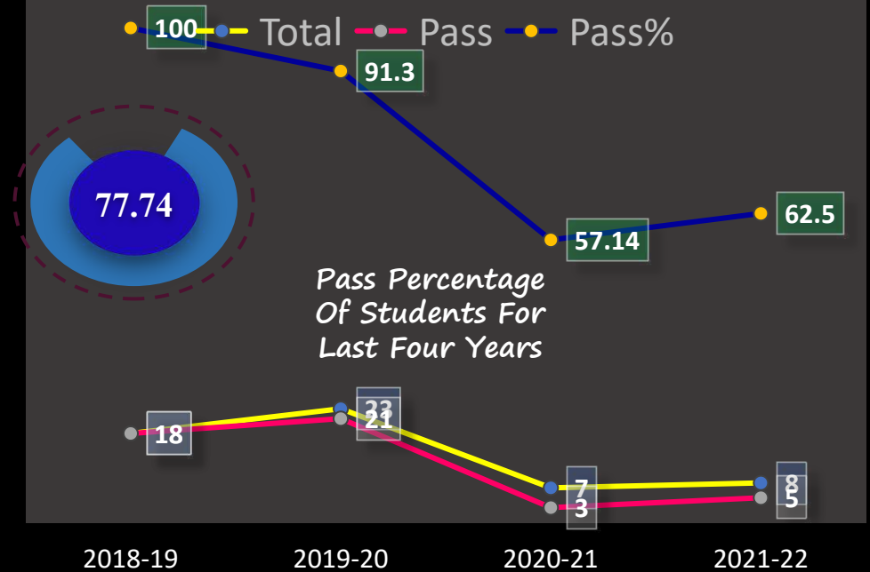
ACADEMIC RESULT ANALYSIS OF PG FROM SESSION 2018-19 TO 2021-22
